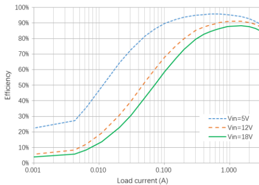
Figure 1. Efficiency vs. Load Current ( V_{OUT}=3.3V , L=2.2\mu H )
