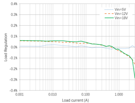
Figure 2. Load Regulation vs. Load Current ( V_{OUT}=3.3V , L=2.2\mu H )
