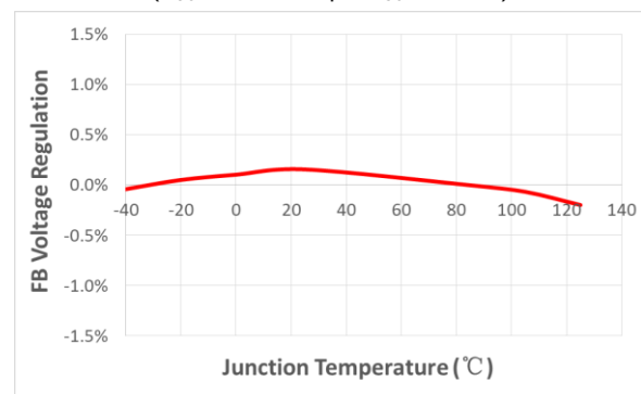
Figure 6. FB Voltage Regulation vs. Junction Temperature
