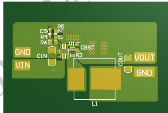
Figure 1. PCB Layout Recommendation
