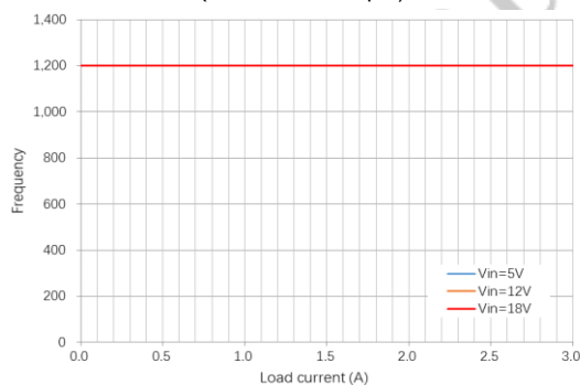
Figure 5. Frequency vs. Load Current ( V_{OUT}=3.3V , L=2.2\mu H )
