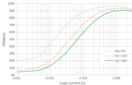
Figure 3. Efficiency vs. Load Current ( V_{OUT}=5V , L=2.2\mu H )
