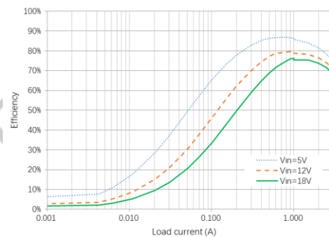
Figure 4. Efficiency vs. Load Current ( V_{OUT}=1V , L=0.68\mu H , C_{OUT}=3*22\mu F )
