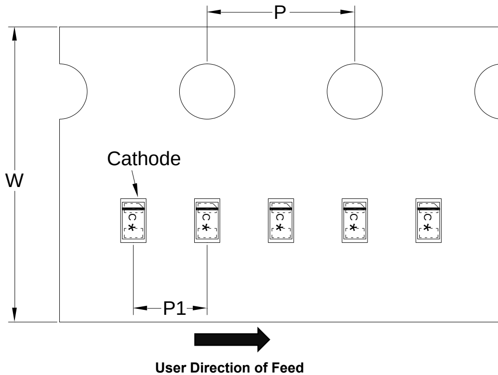
Tape Dimensions
