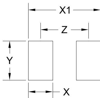
Land Layout
