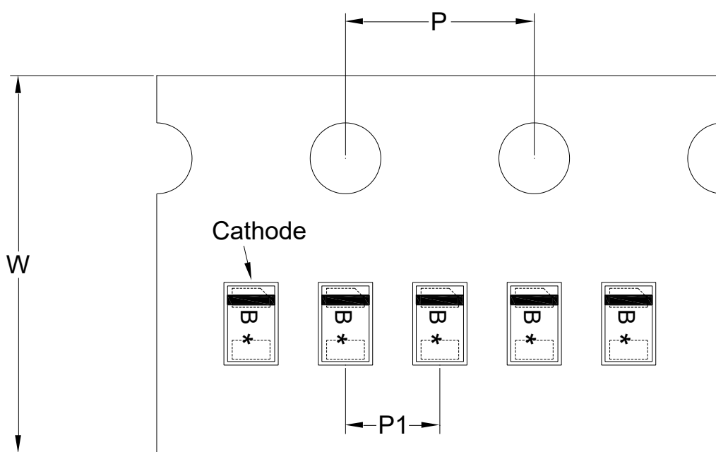
Tape Dimensions
