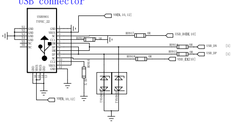
USB connector
