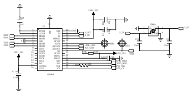
SPI接口CH390H
